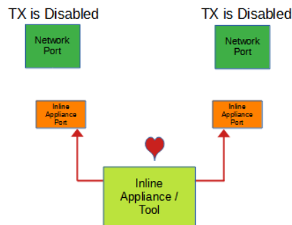
Figure 7 Default Tap Mode (Reverse Bypass)
